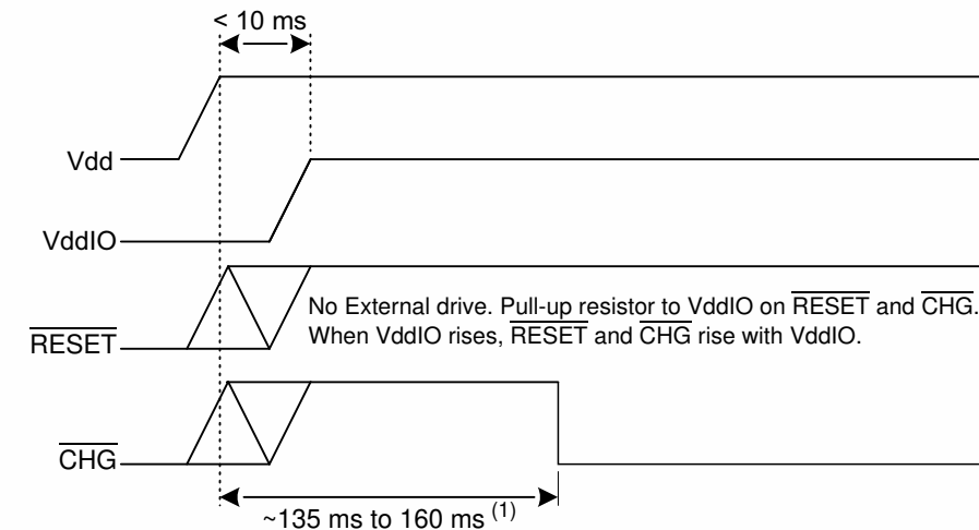
FIGURE 5-3: POWER-UP SEQUENCE
