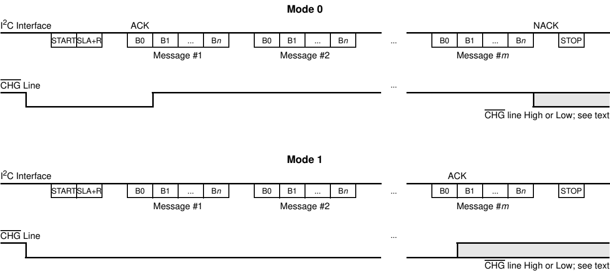
FIGURE 7-12: CHG LINE MODES FOR I 2 C-COMPATIBLE TRANSFERS
