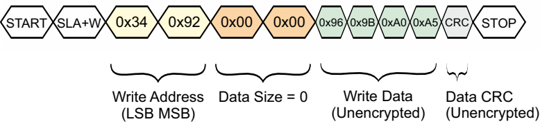
FIGURE 7-4: EXAMPLE OF A WRITE TO ADDRESS 0x1234 WITH A CHECKSUM – ENCRYPTION ACTIVE
