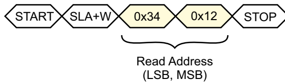
FIGURE 7-5: EXAMPLE OF A FOUR-BYTE READ – ENCRYPTION NOT ACTIVE
