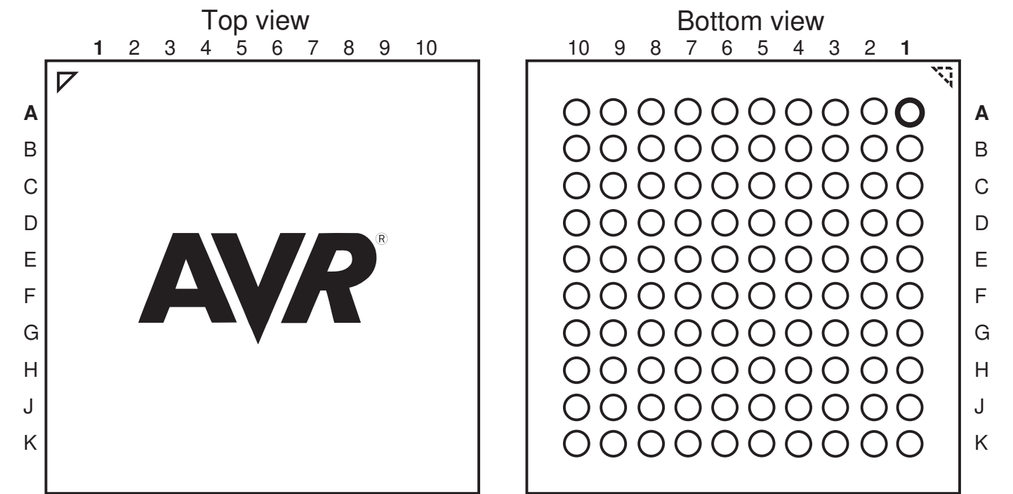
Figure 1-2. CBGA-pinout ATmega640/1280/2560
