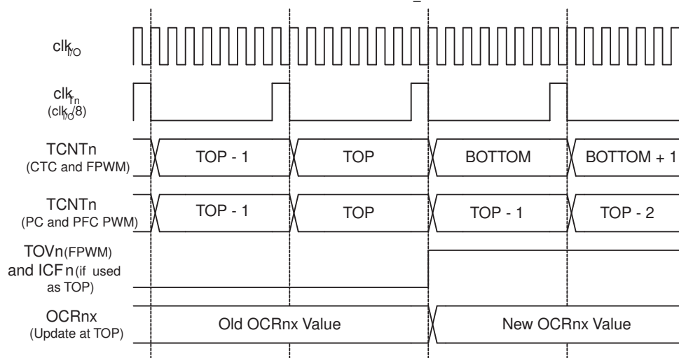
Figure 17-13. Timer/Counter Timing Diagram, with Prescaler ( f_{\text{clk\_I/O}}/8 )
