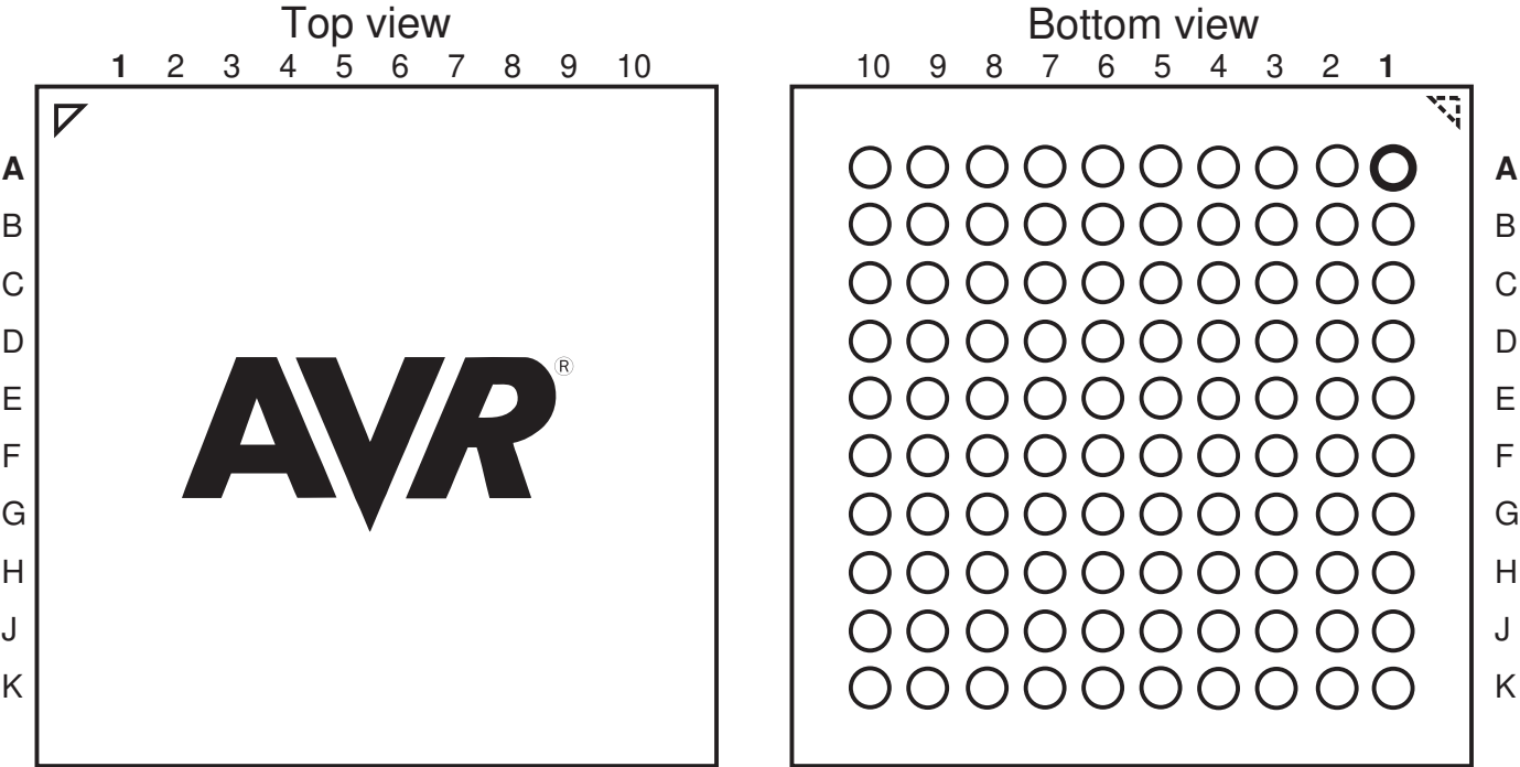
Figure 1-2. CBGA-pinout ATmega640/1280/2560
