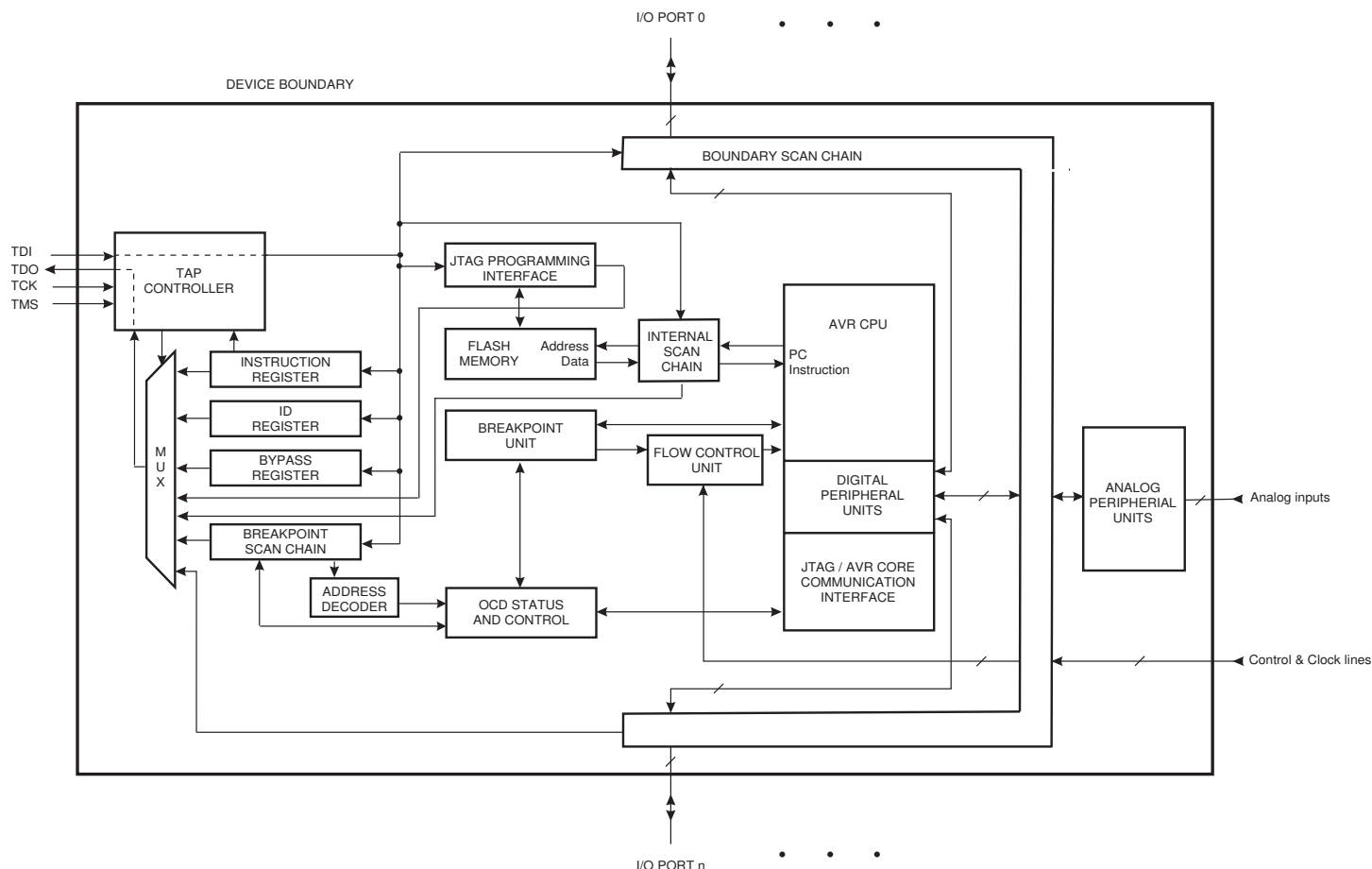
Figure 27-1. Block Diagram
