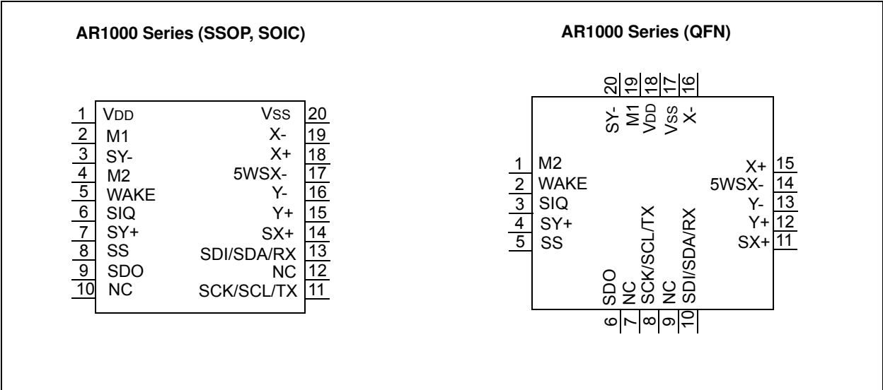
FIGURE 1-2: PIN DIAGRAM
