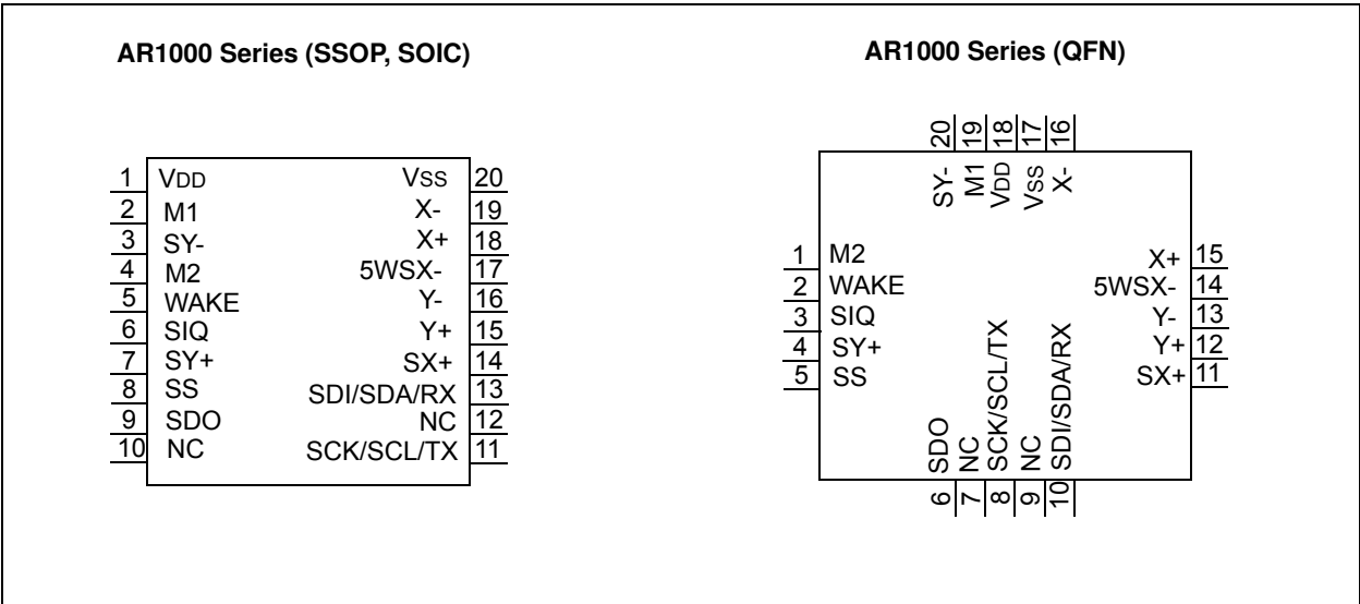
FIGURE 1-2: PIN DIAGRAM
