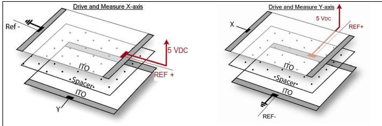
FIGURE 2-2: 8-WIRE DECODING
