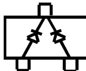
Common Cathode
