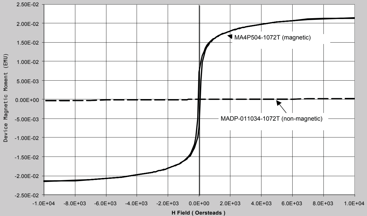
Comparison of Magnetic Moment vs. H Field for MA4P504-1072T & MADP-011034-1072T
