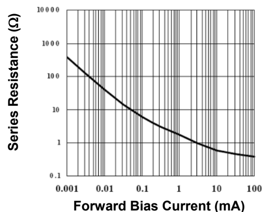
Resistance vs. Forward Current (MA4P7433/ MADP-007433 Series)
