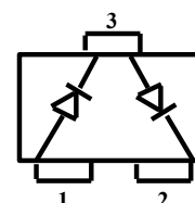
Series Pair MA4E1339B-287T MA4E1339B-1146T
