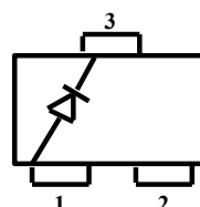
Single MA4E1339A-287T MA4E1339A-1146T
