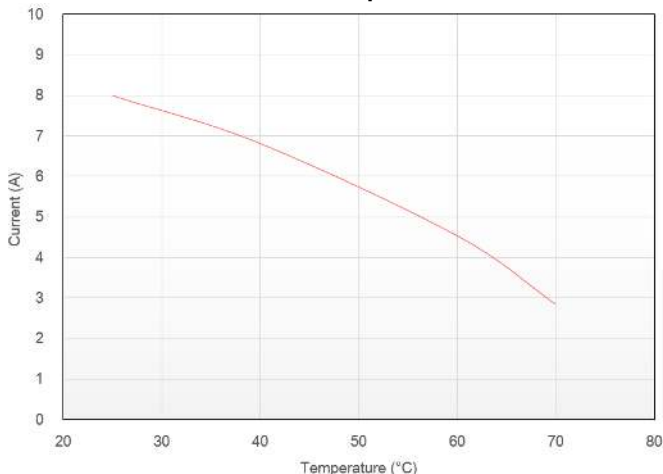
Hold Current vs. Temperature Curve
