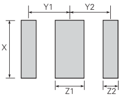
Pad Layout - Surface-mount Devices (GTCS35-XXXXM-R05)
