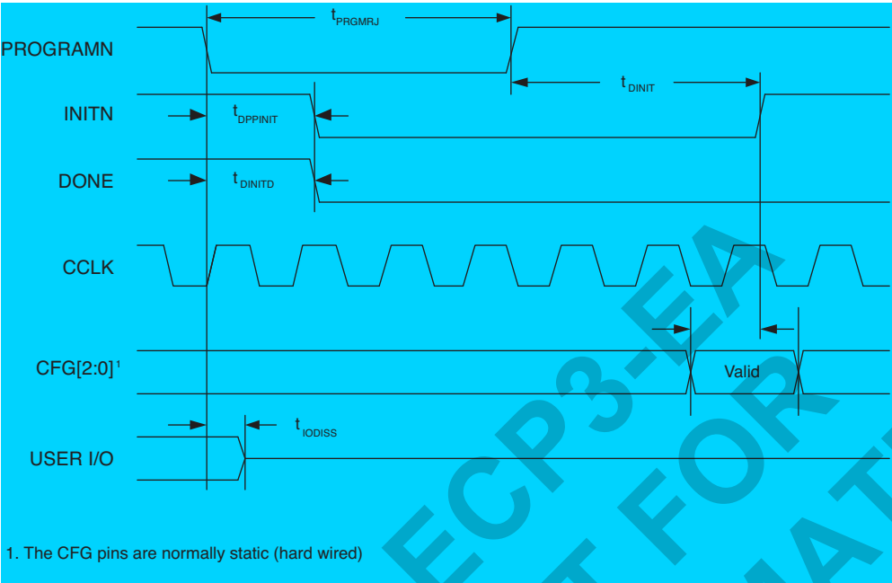
Figure 3-23. Wake-Up Timing
