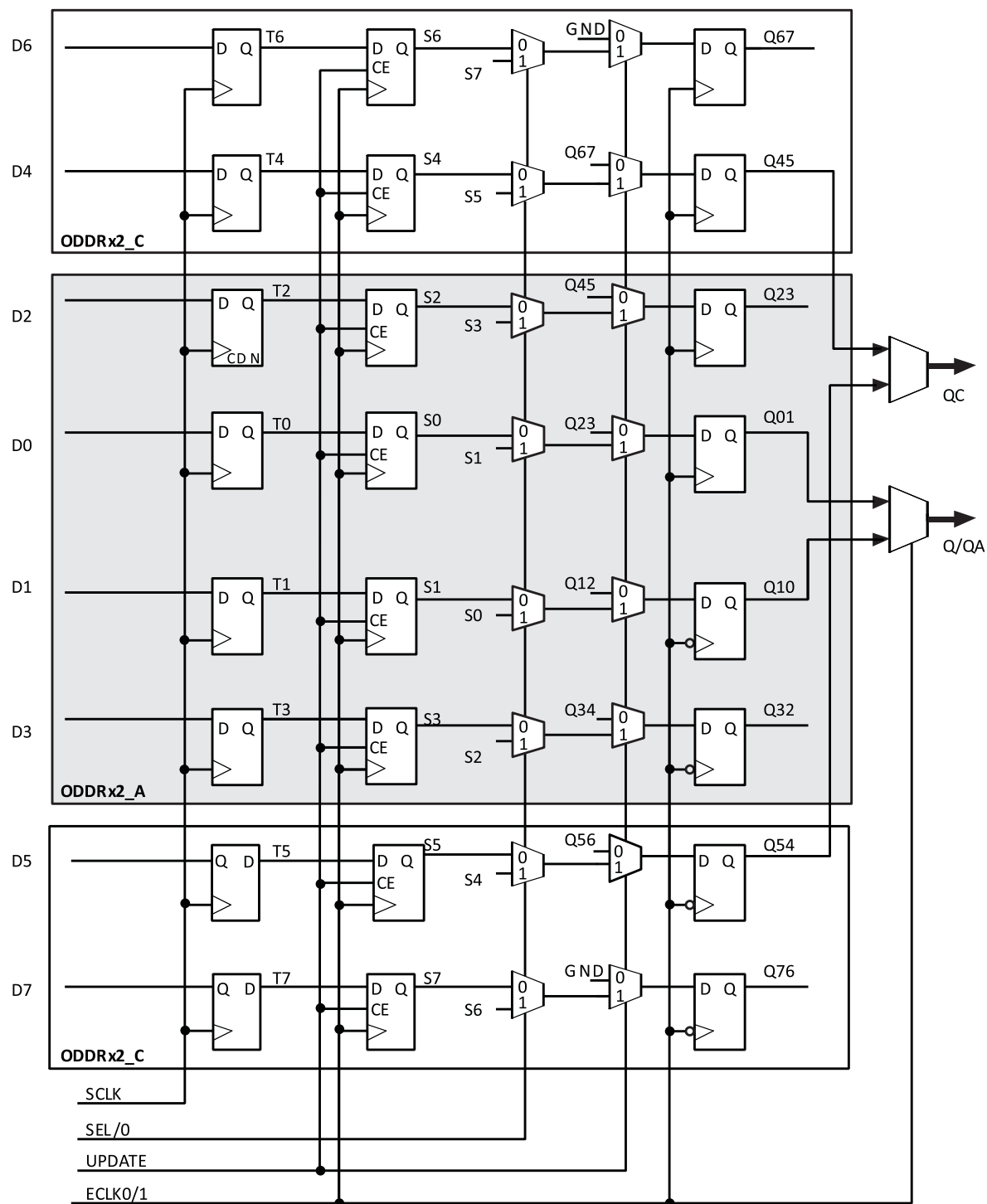
Figure 2.14. Output Gearbox
