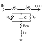
Electrical Model
