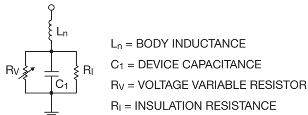
Figure 4. Antenna Varistor
