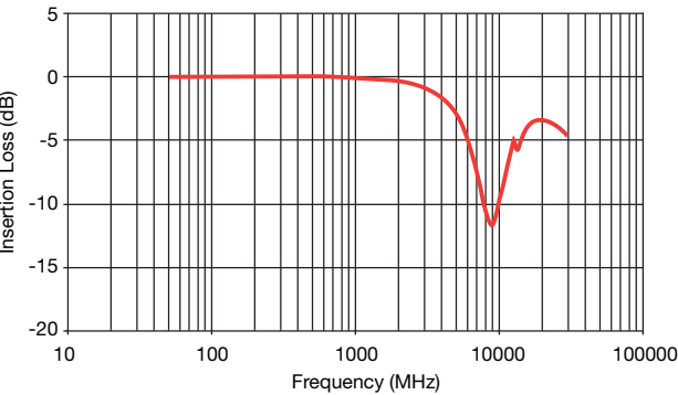
S21 TRANSMISSION CHARACTERISTICS
