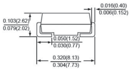
SMC/DO-214AB
