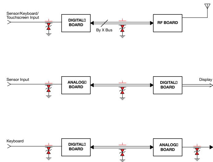
Fig. 1 – System Interface
