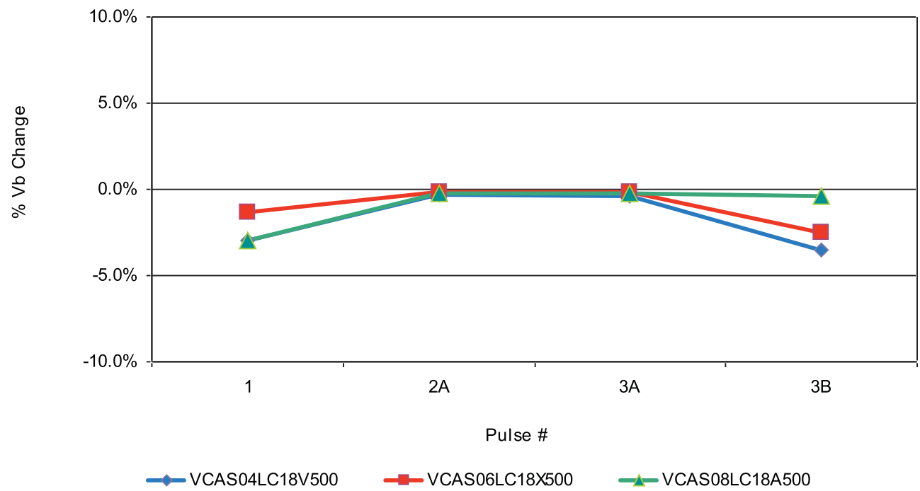
ISO 7637 Pulse 1-3
