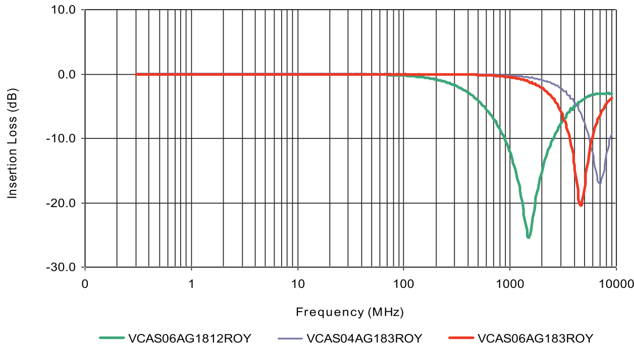
S21 Response
