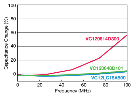
TransGuard® Capacitance vs Frequency 1206
