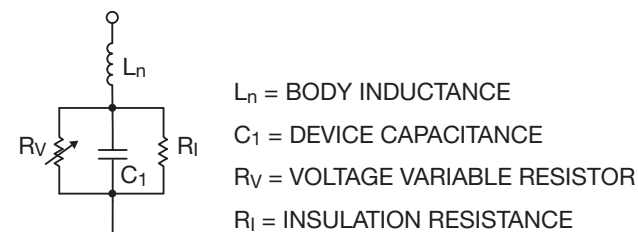
Figure 4. Antenna Varistor
