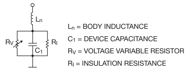
Figure 4. Antenna Varistor
