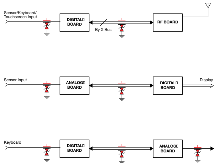
Fig. 1 – System Interface
