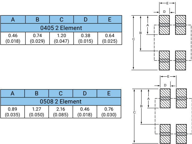
PAD LAYOUT DIMENSIONSmm (inches)
