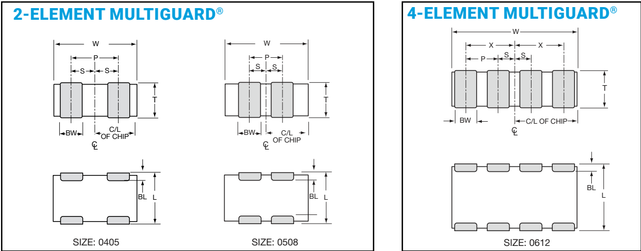
0405 2 ELEMENT DIMENSIONSmm (inches)
