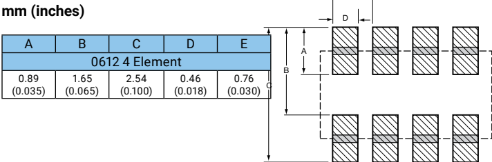
PAD LAYOUT DIMENSIONS
