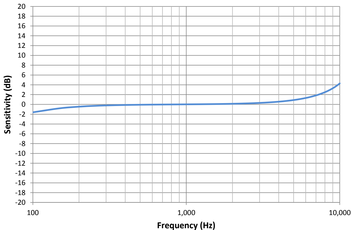
Typical Free Field Response Normalized to 1 kHz ( C1 = 2.2\mu\text{F} )
