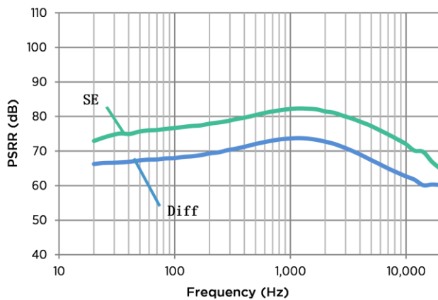
Figure 9: Typical PSRR (LPM)
