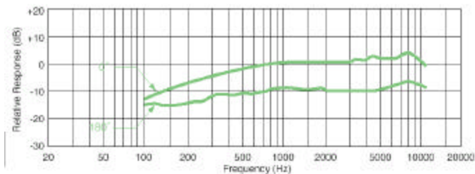
Frequency Response Curve
