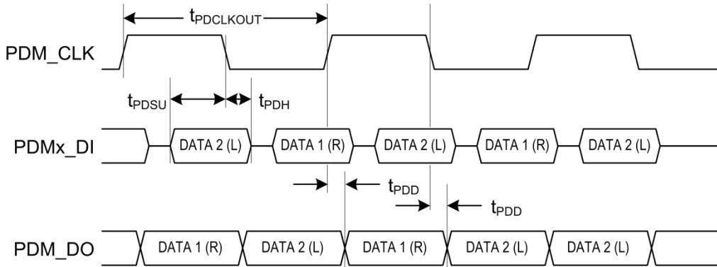
Figure 17 PDM Interface Timing
