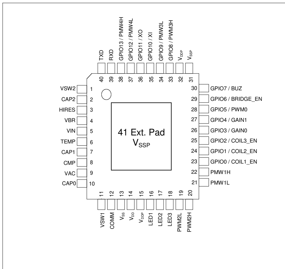
Figure 7 XMCXXXXSC PG-VQFN-40-17 Pin Configuration (top view)
