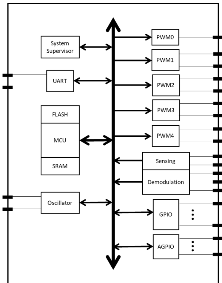
Figure 1 Block Diagram
