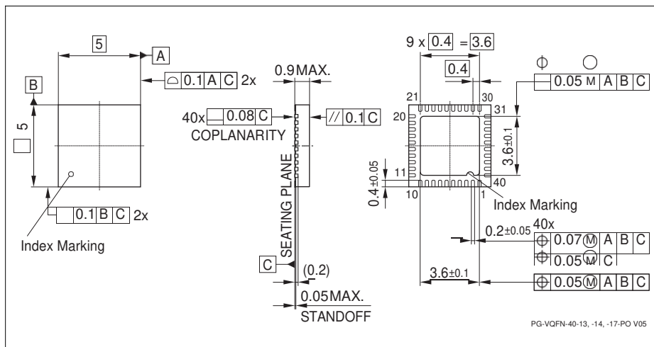
Figure 30 PG-VQFN-40-17
