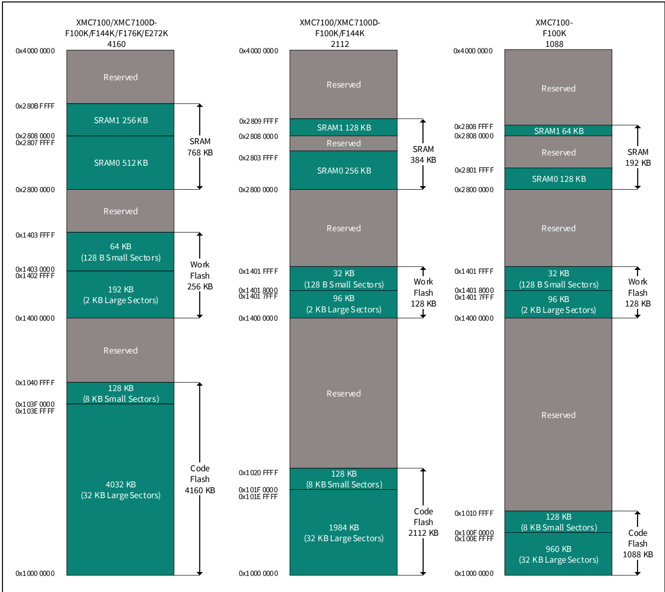
Figure 4 XMC7100 address map 2 [25]
