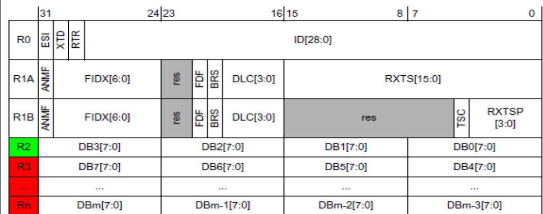
Figure 1 RX buffer and FIFO element
