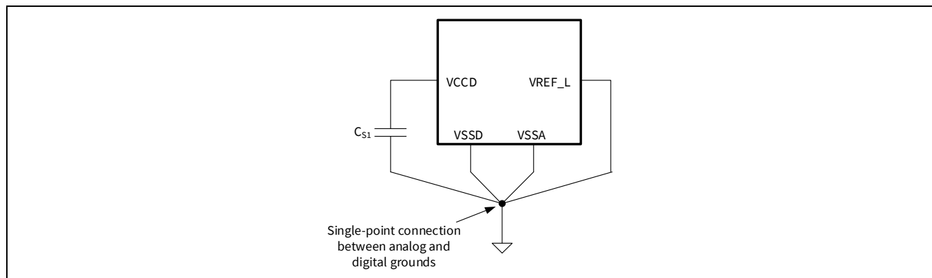
Figure 16 Smoothing capacitor
