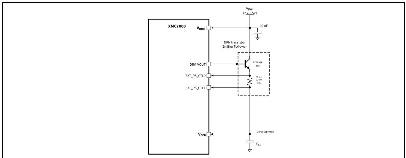
Figure 1 Sample core external regulator with NPN transistor
