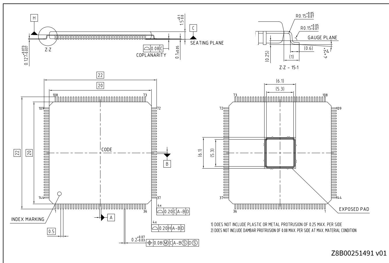
Figure 63 144-pin TEQFP (20.0 × 20.0 × 1.6 mm) LEL144 (PG-TQFP-144), package outline
