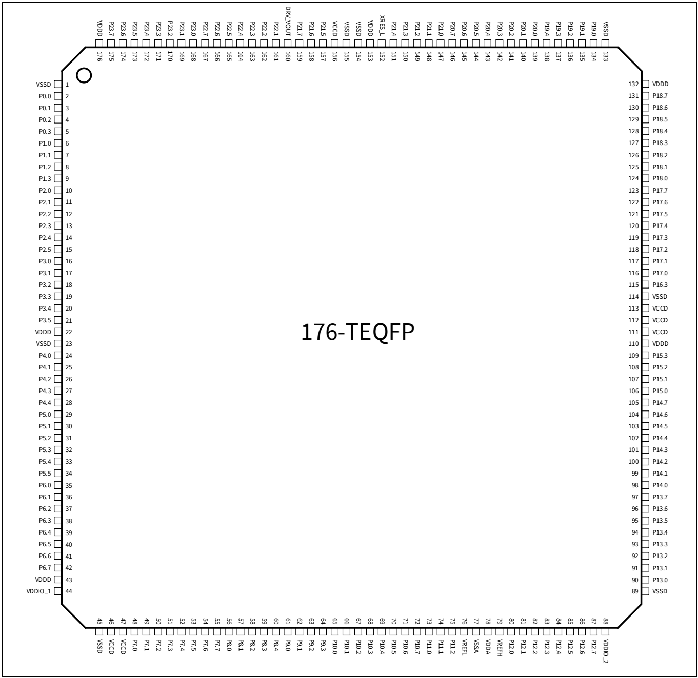
Figure 10 176-TEQFP pin assignment
