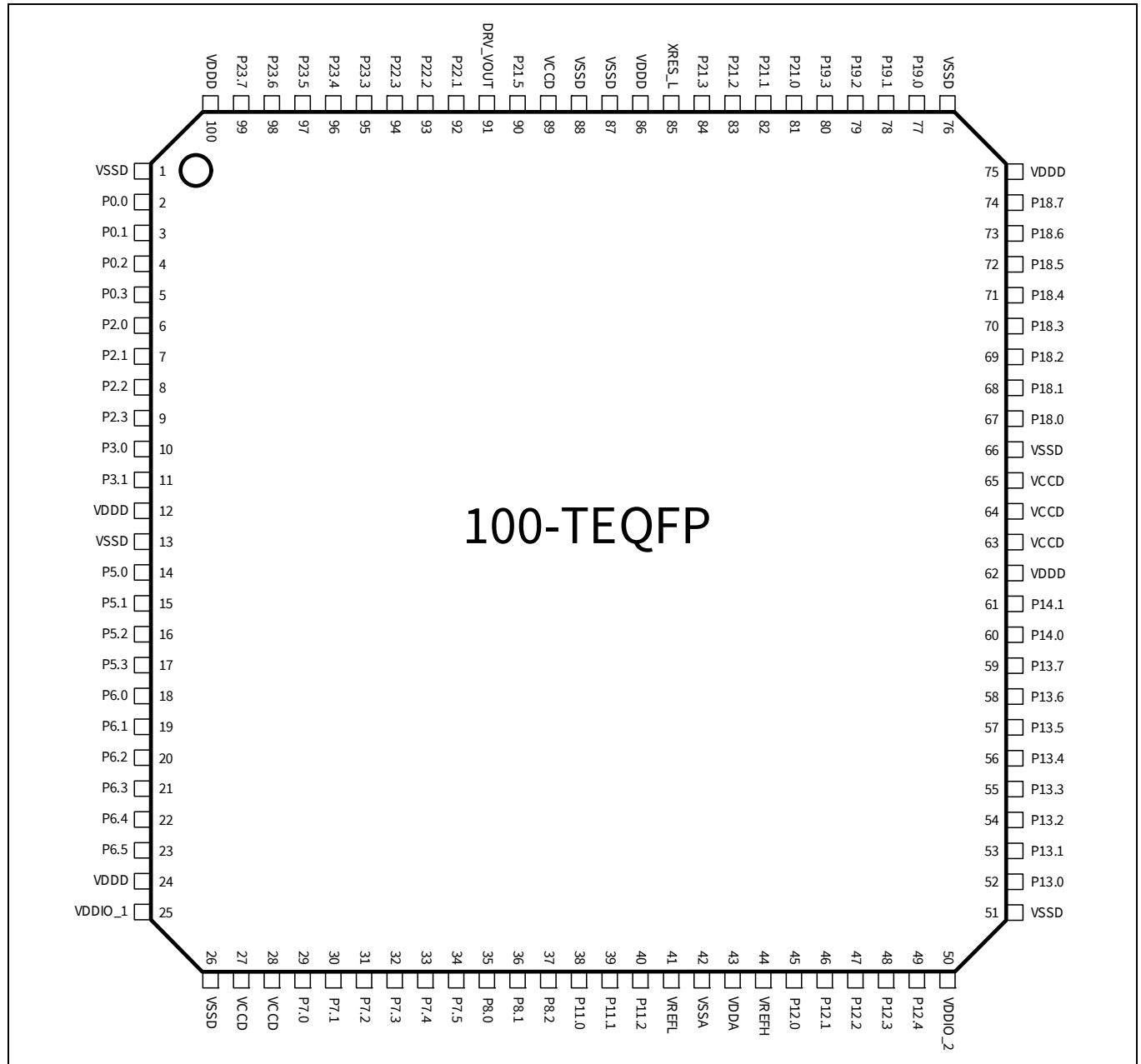
Figure 6 100-TEQFP pin assignment
