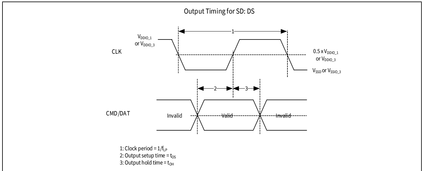
Figure 44 SD default speed output timing
