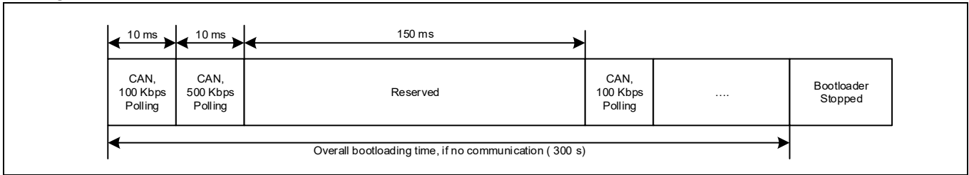
Figure 66 Bootloading sequence
