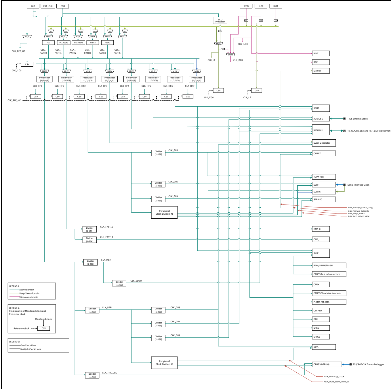
Figure 5 XMC7100 clock diagram
