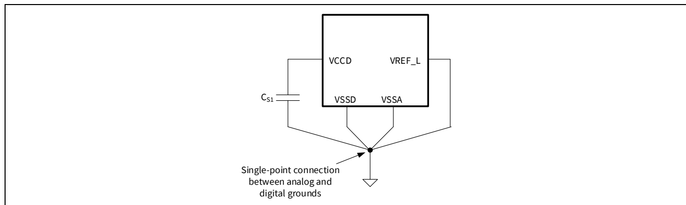
Figure 16 Smoothing capacitor
