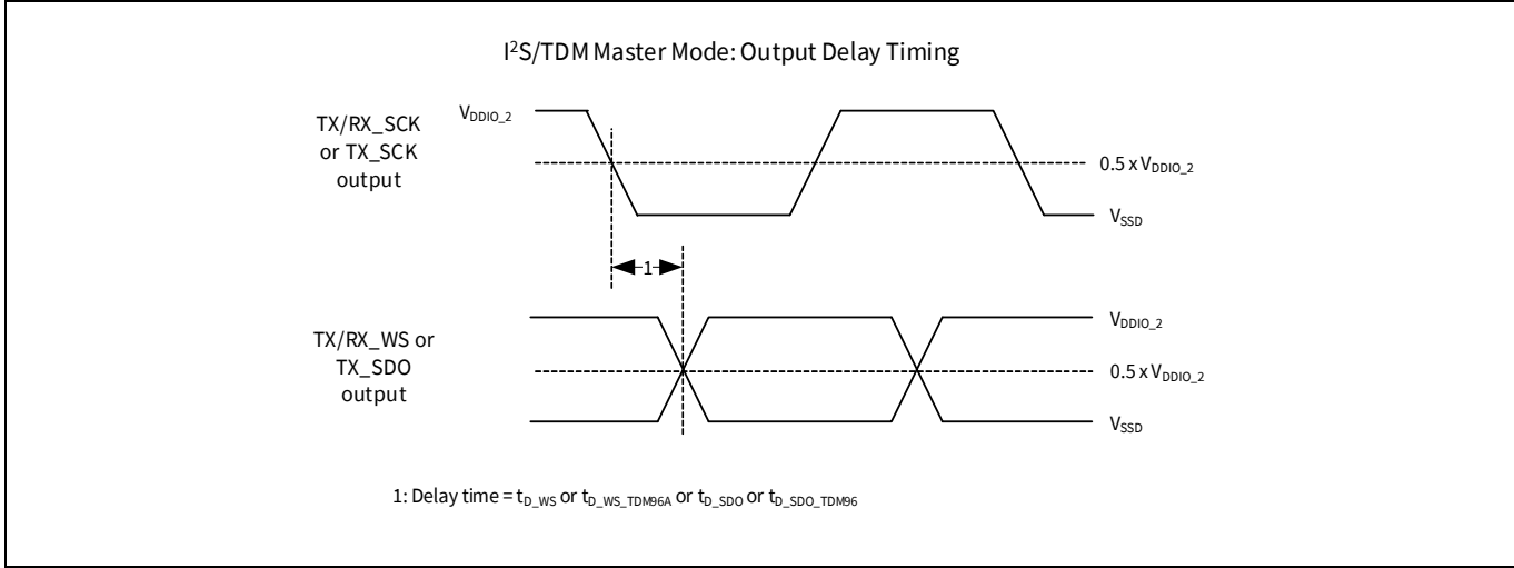
Figure 49 Master output delay
