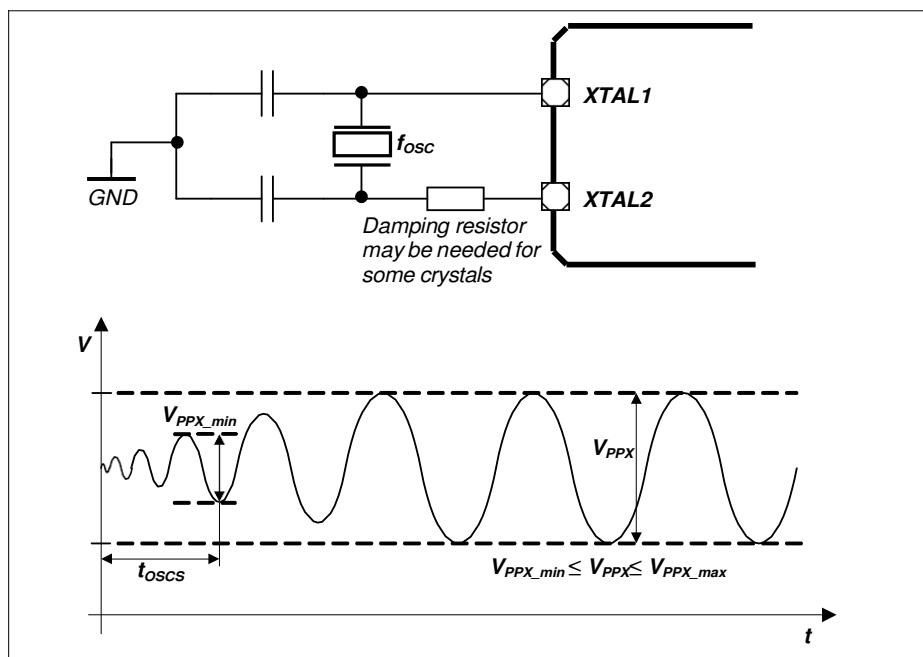
Figure 15 Oscillator in Crystal Mode
