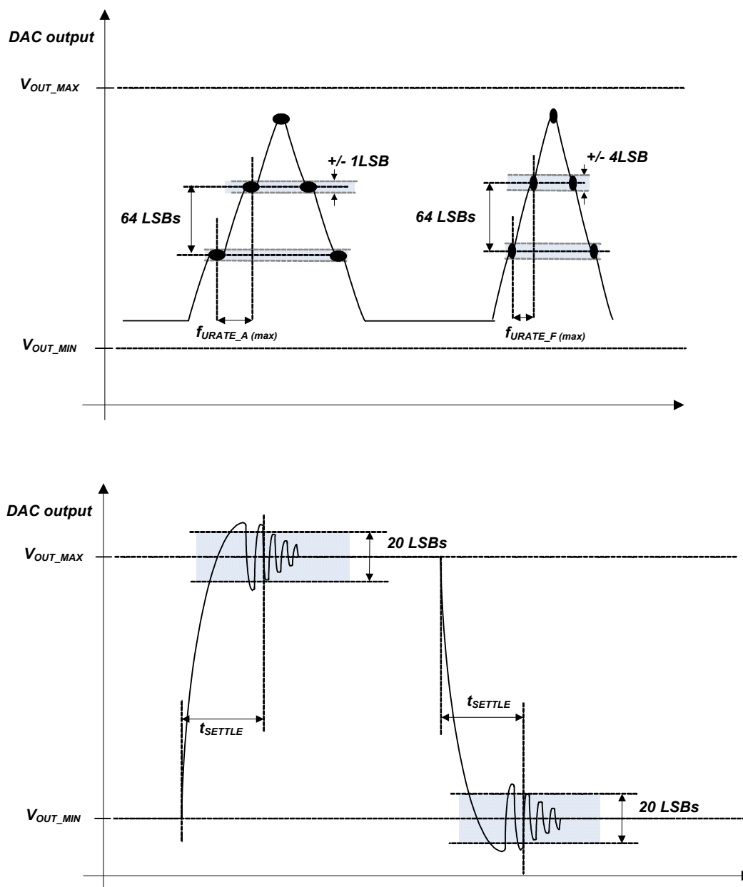
Figure 17 DAC Conversion Examples
