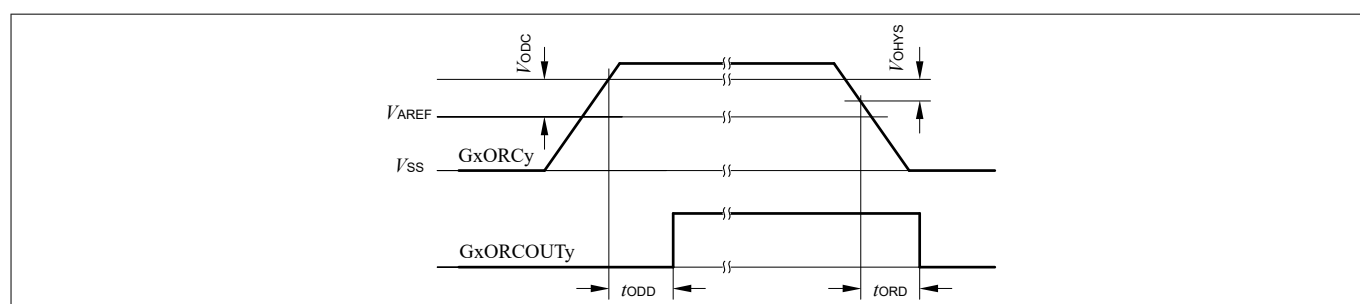
Figure 18 GxORCOUTy Trigger Generation
