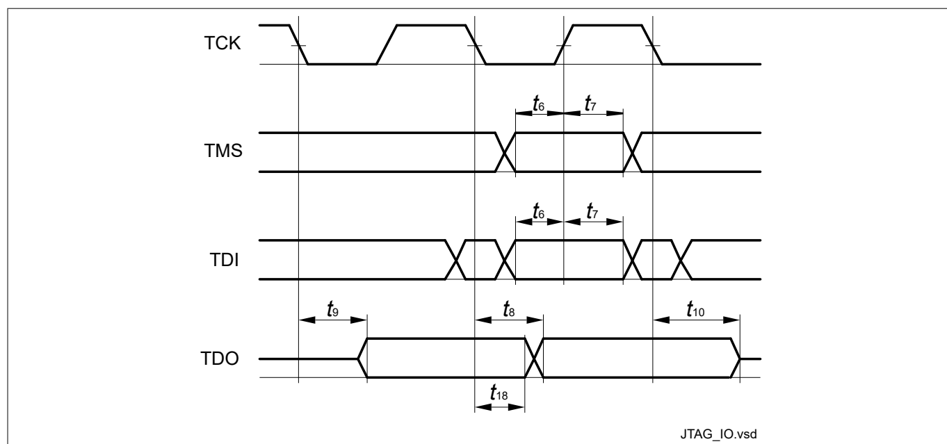
Figure 28 JTAG Timing
