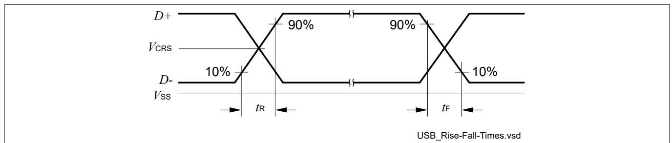
Figure 38 USB Signal Timing
