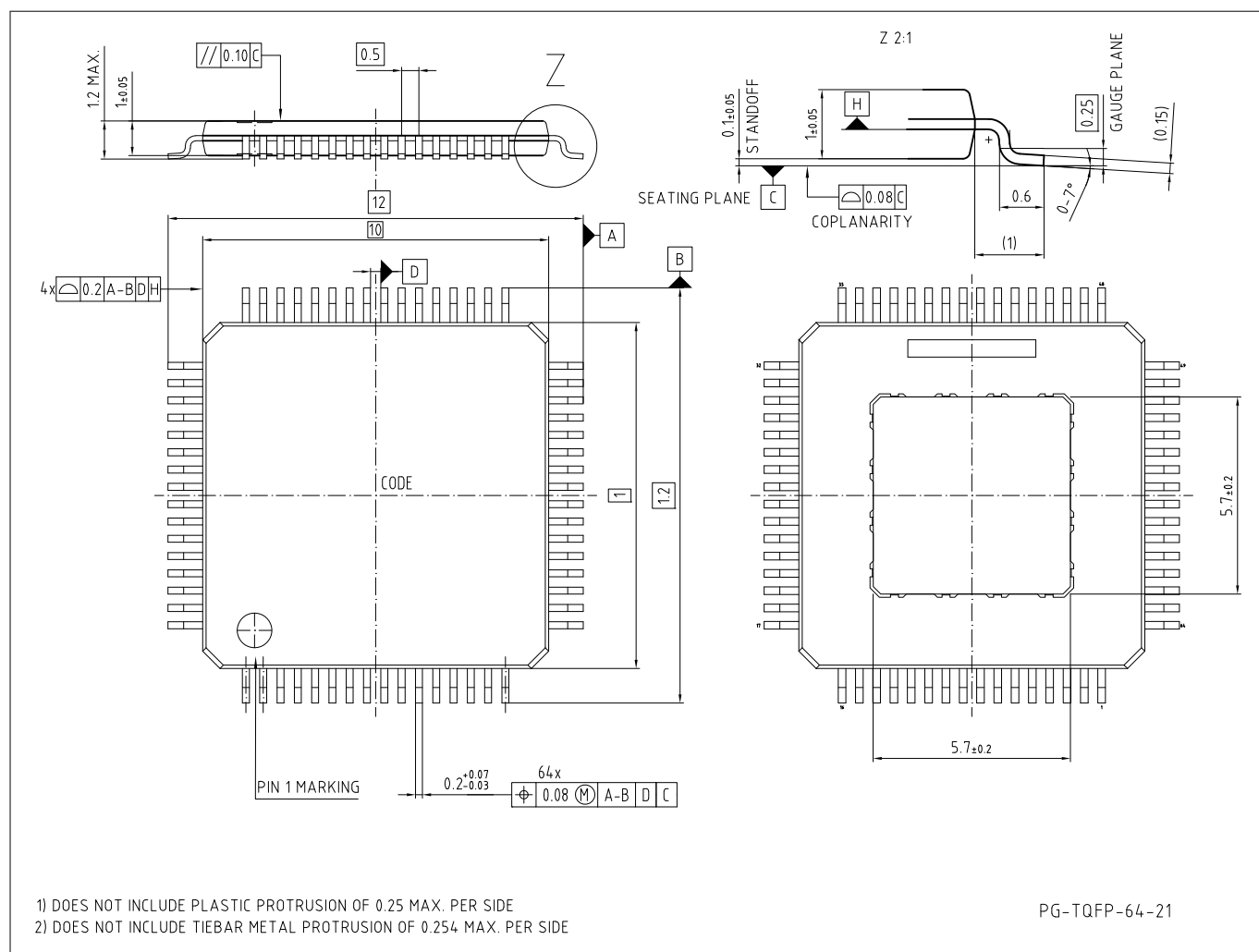
Figure 45 PG-TQFP-64-21 (Plastic Green Low Profile Quad Flat Package)
