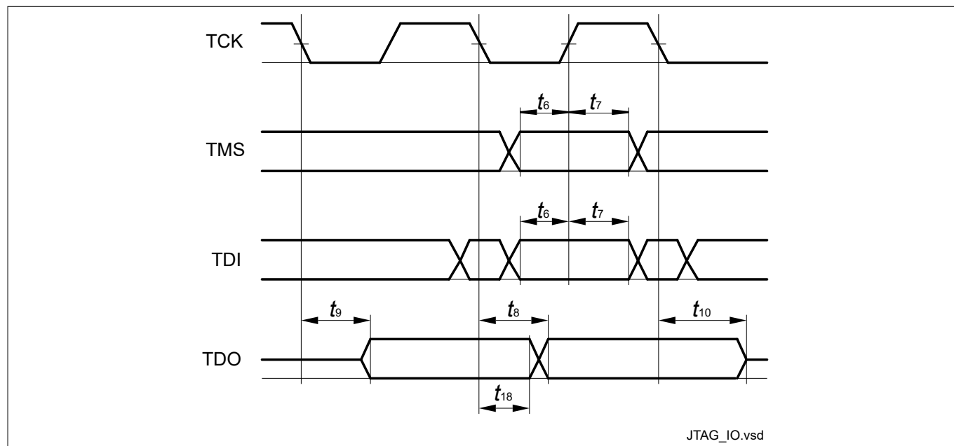
Figure 29 JTAG Timing
