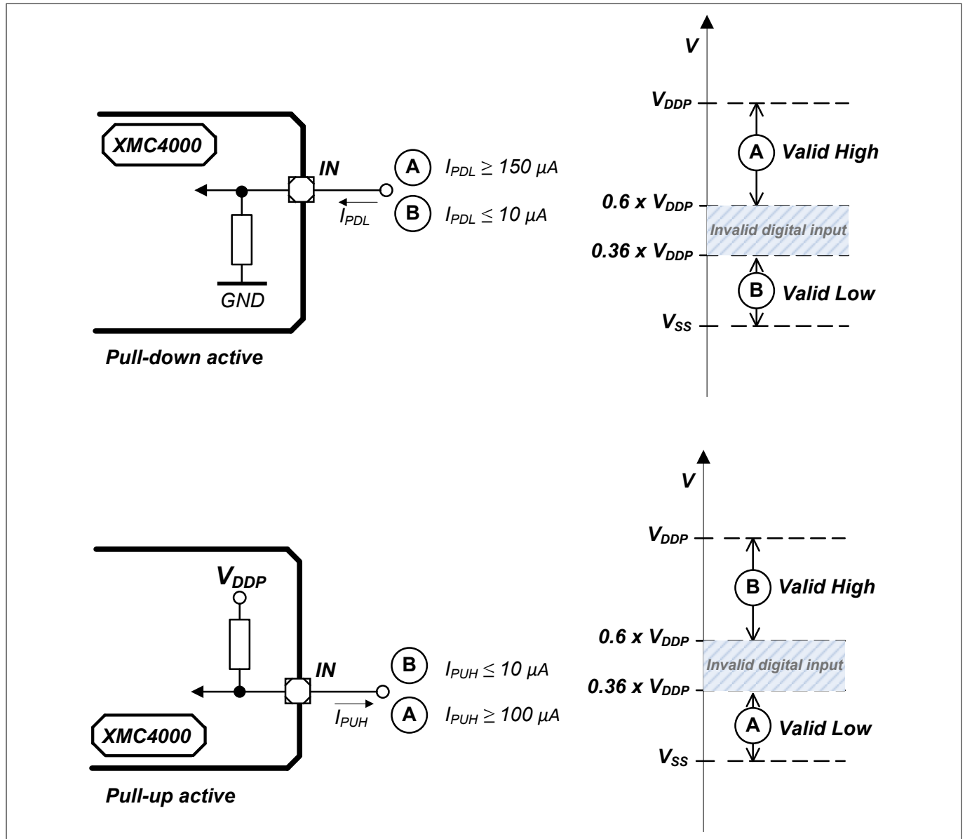
Figure 11 Pull Device Input Characteristics
