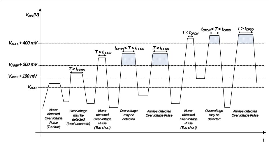
Figure 16 GxORCOUTy Trigger Generation
