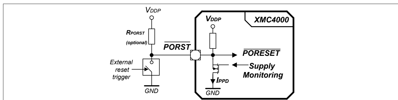
Figure 26 \overline{\text{PORST}} Circuit
