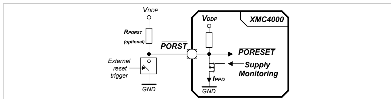
Figure 26 PORST Circuit
