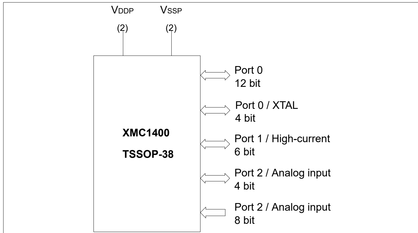
Figure 2 XMC1400 Logic Symbol for TSSOP-38-9
