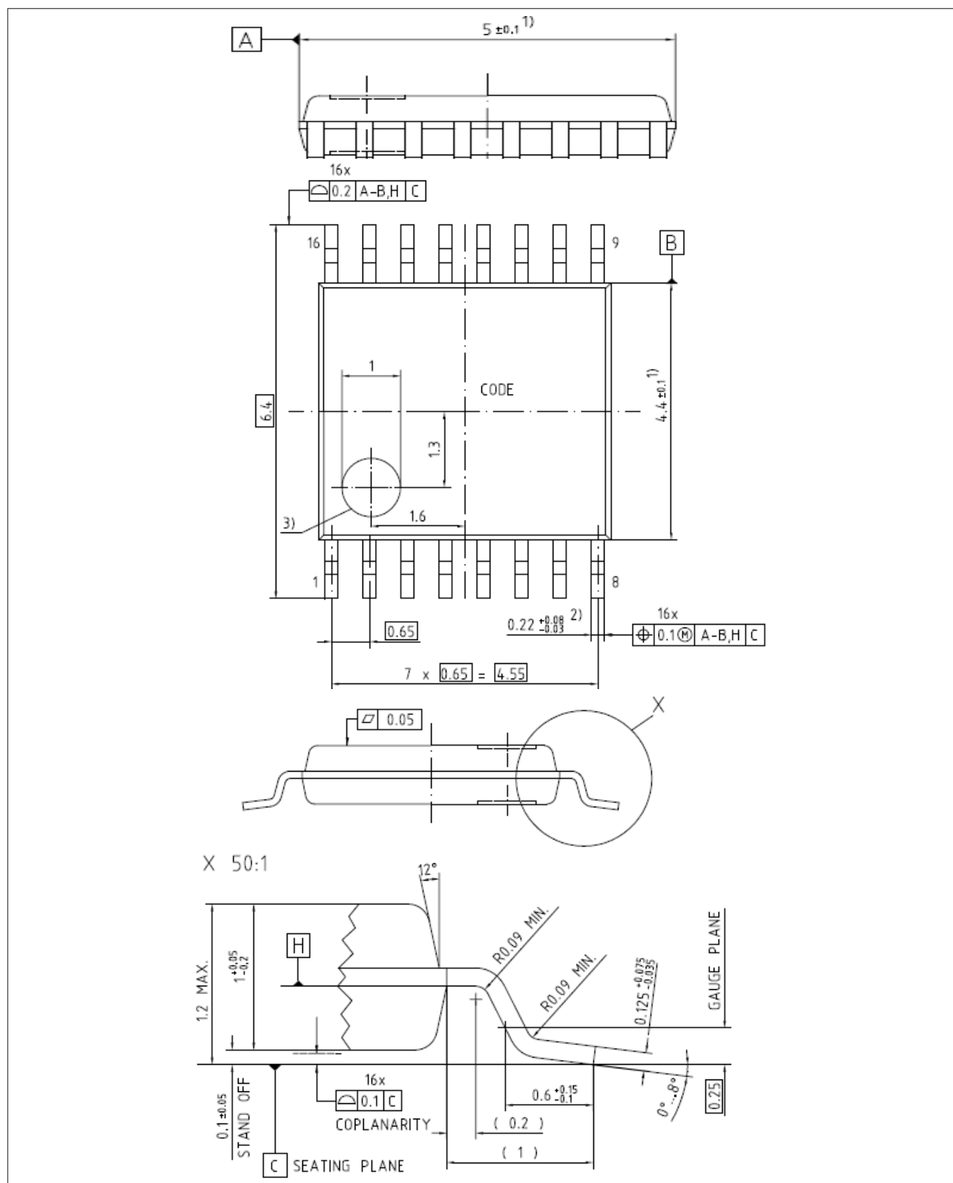
Figure 28 PG-TSSOP-16-8
