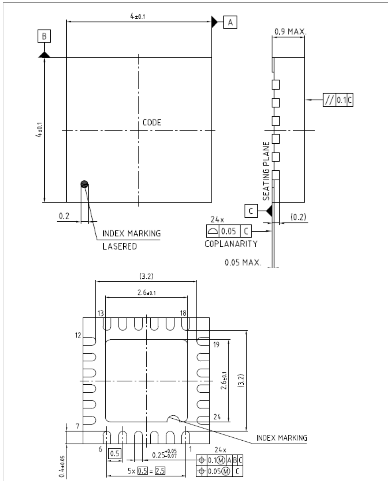
Figure 29 PG-VQFN-24-19
