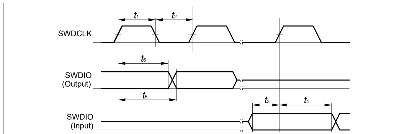
Figure 21 SWD Timing
