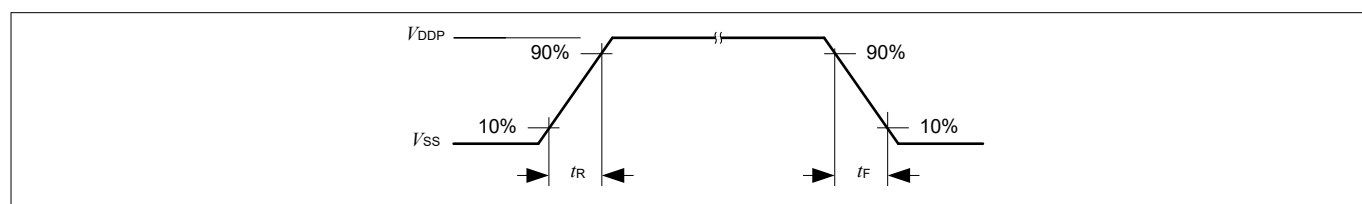
Figure 16 Rise/Fall Time Parameters
