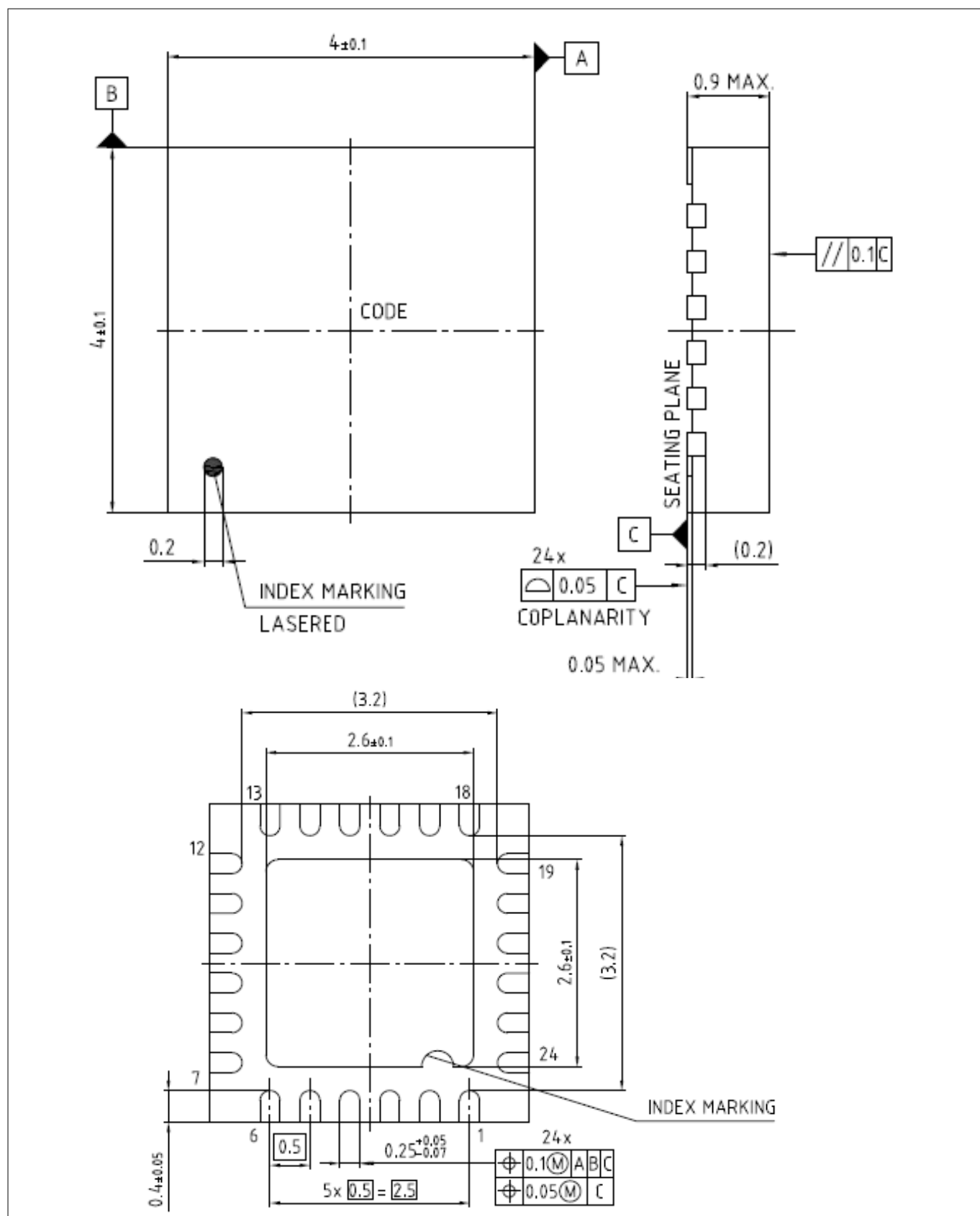
Figure 29 PG-VQFN-24-19
