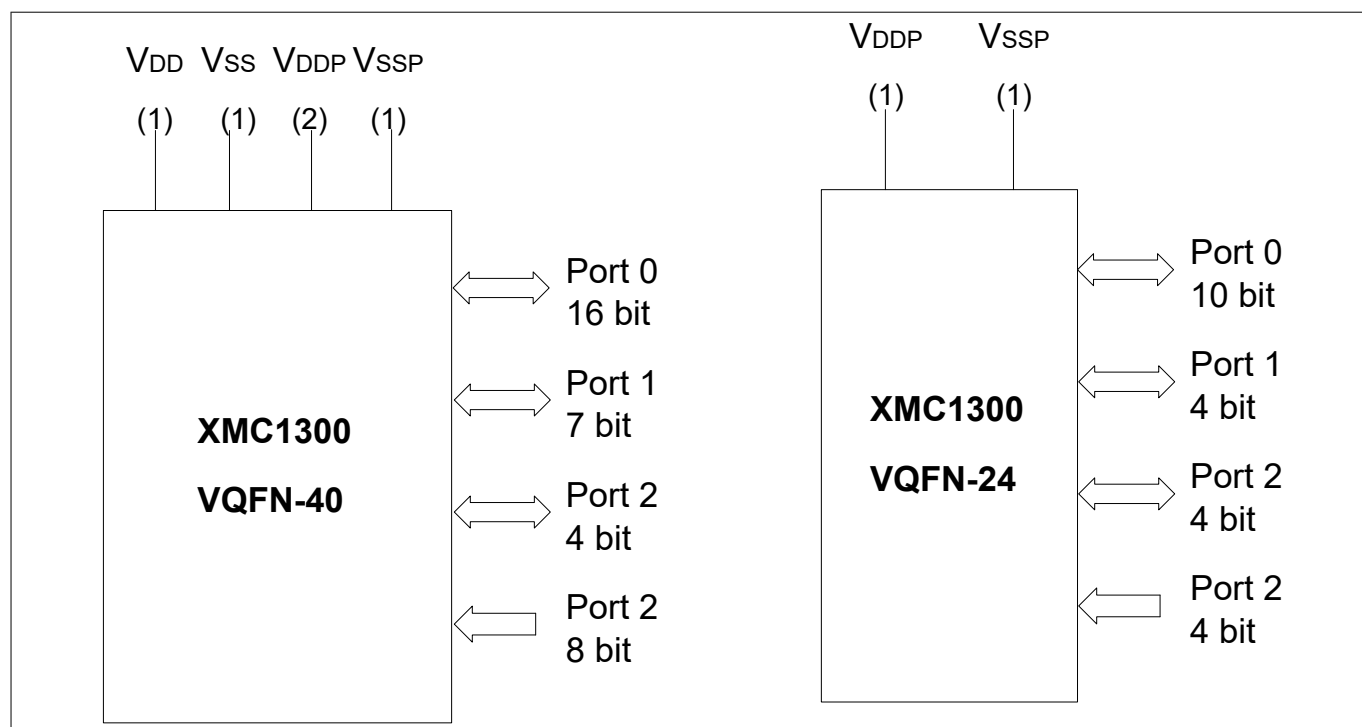
Figure 3 XMC1300 Logic Symbol for VQFN-24 and VQFN-40
