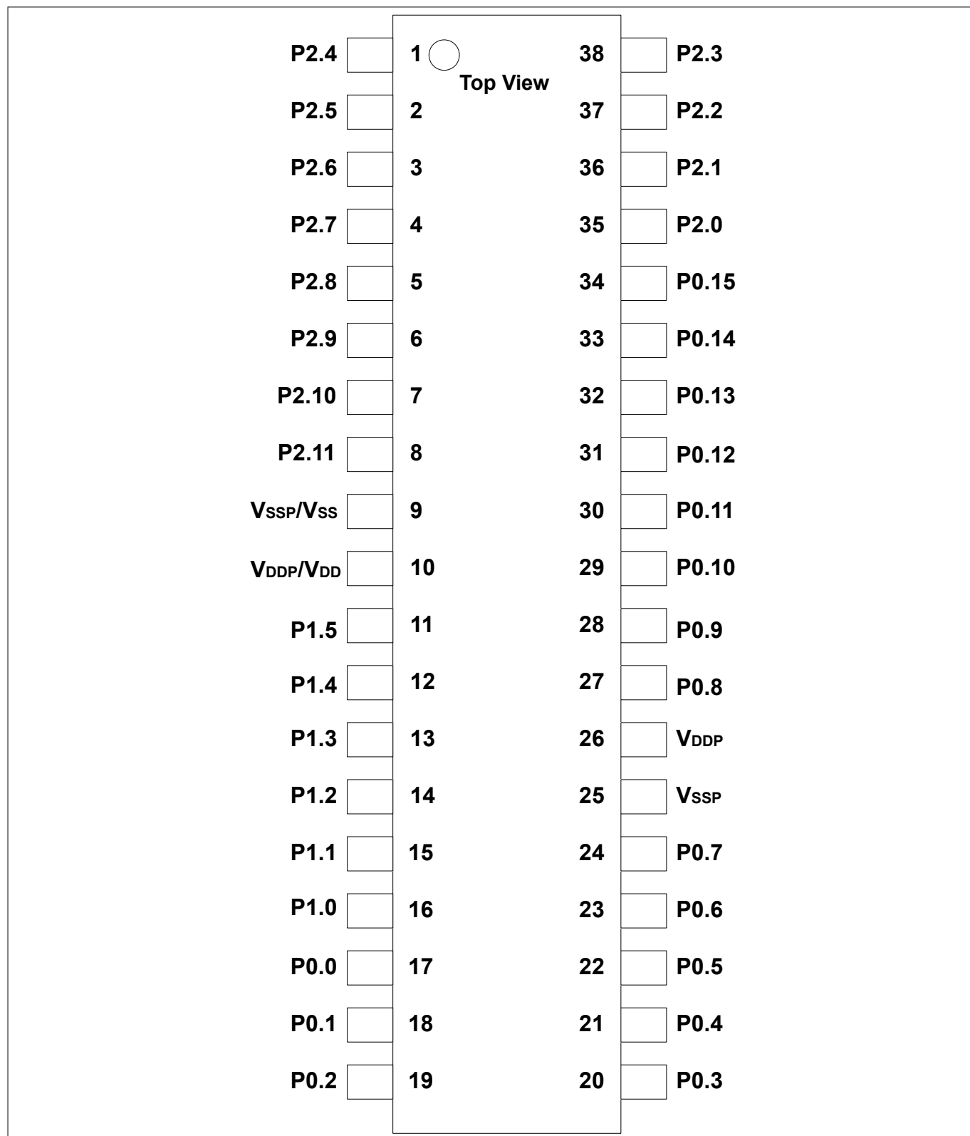
Figure 4 XMC1300 PG-TSSOP-38 Pin Configuration (top view)
