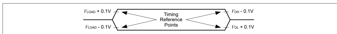
Figure 18 Testing Waveform, Output High Impedance
