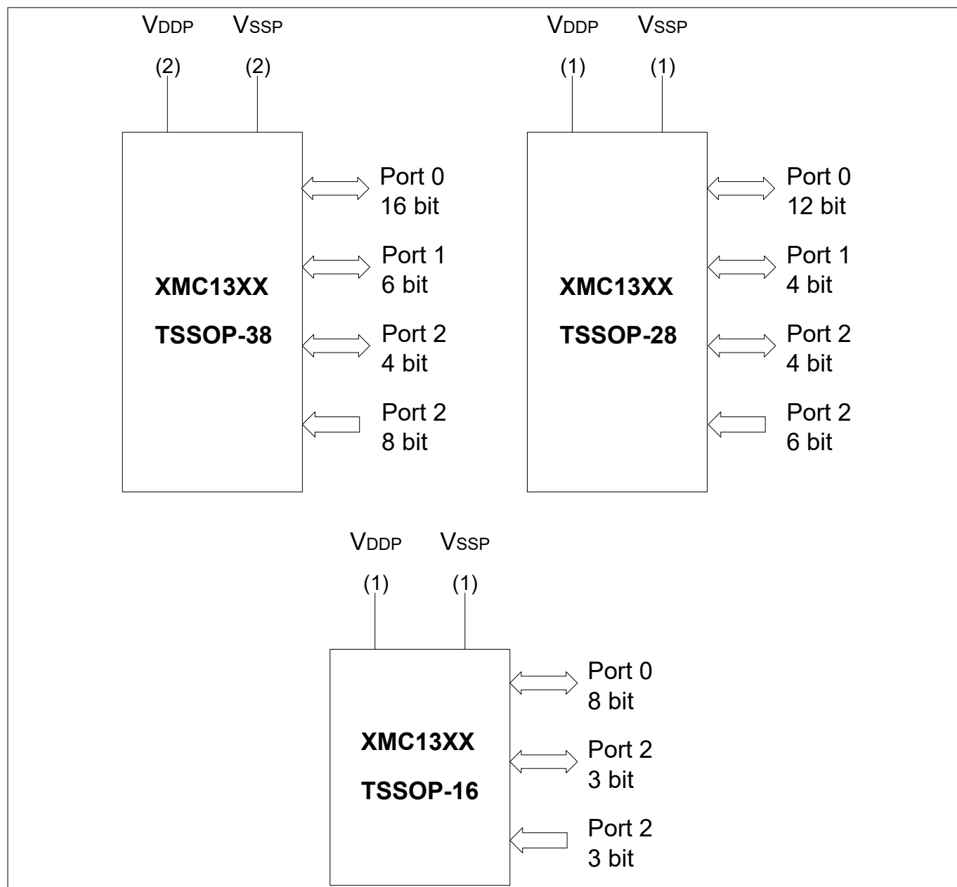
Figure 2 XMC1300 Logic Symbol for TSSOP-38, TSSOP-28 and TSSOP-16
