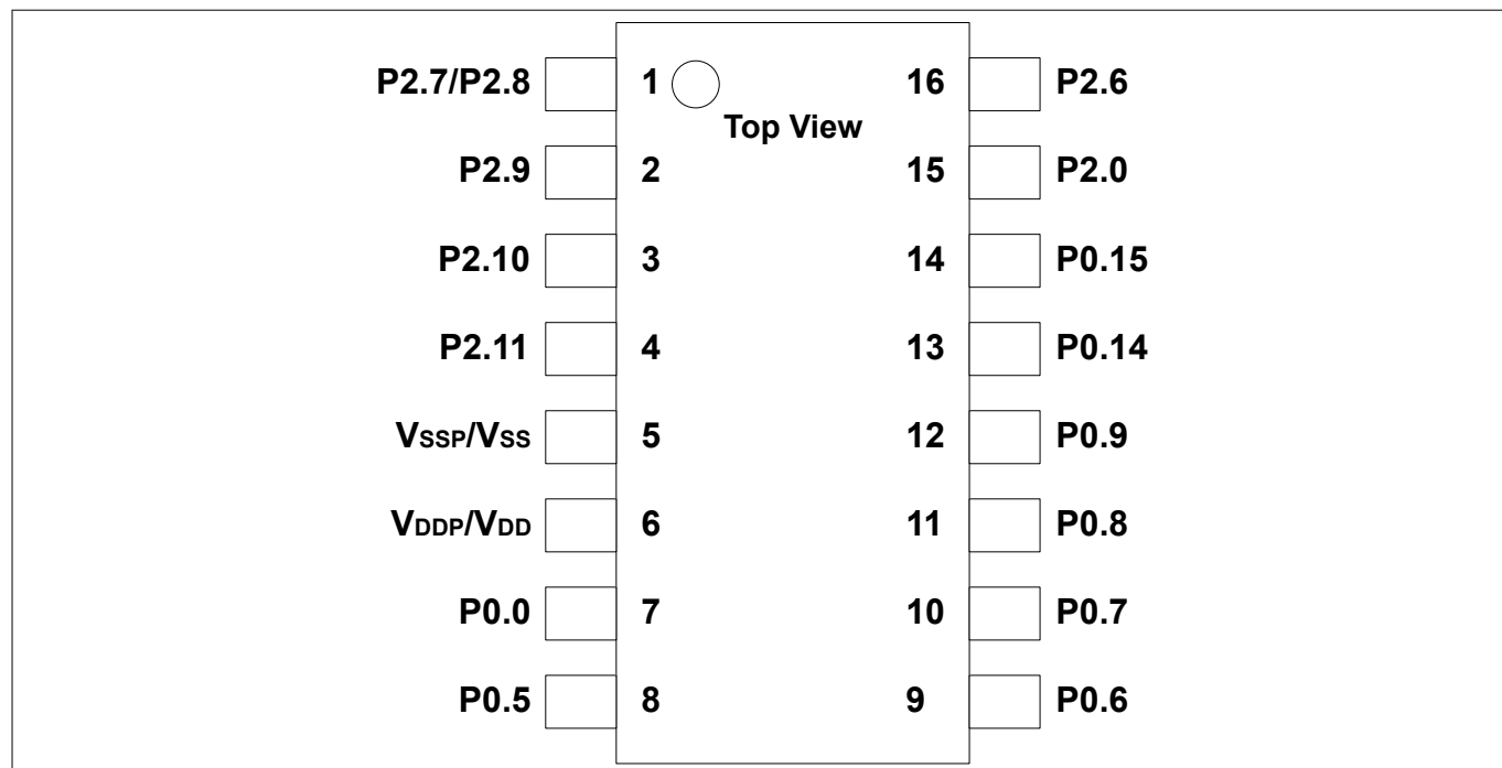
Figure 6 XMC1300 PG-TSSOP-16 Pin Configuration (top view)
