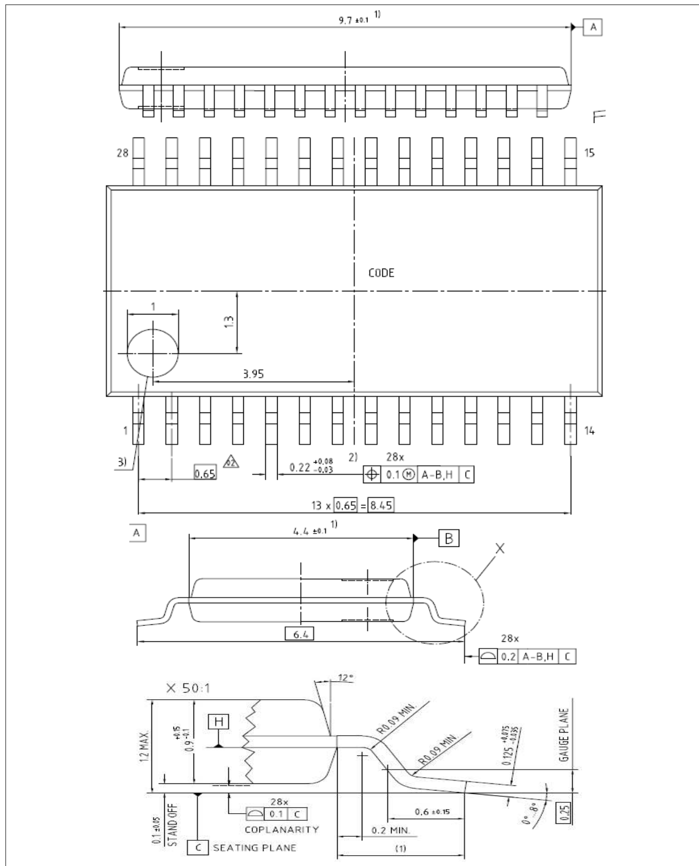
Figure 27 PG-TSSOP-28-16
