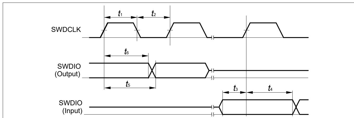
Figure 21 SWD Timing
