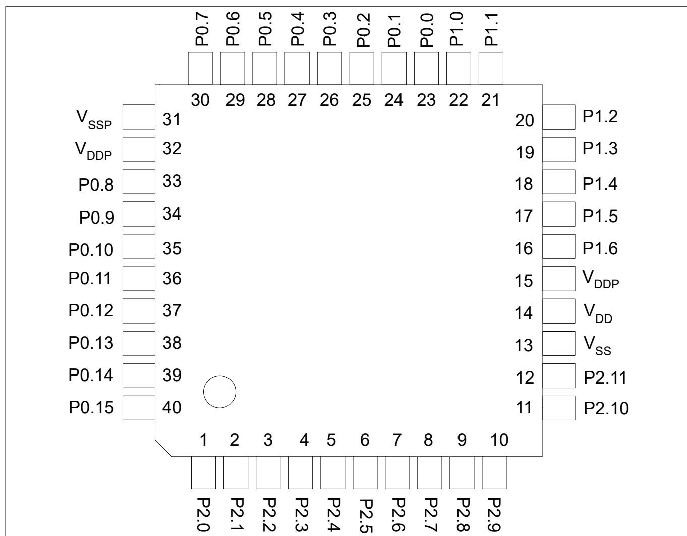
Figure 8 XMC1300 PG-VQFN-40 Pin Configuration (top view)
