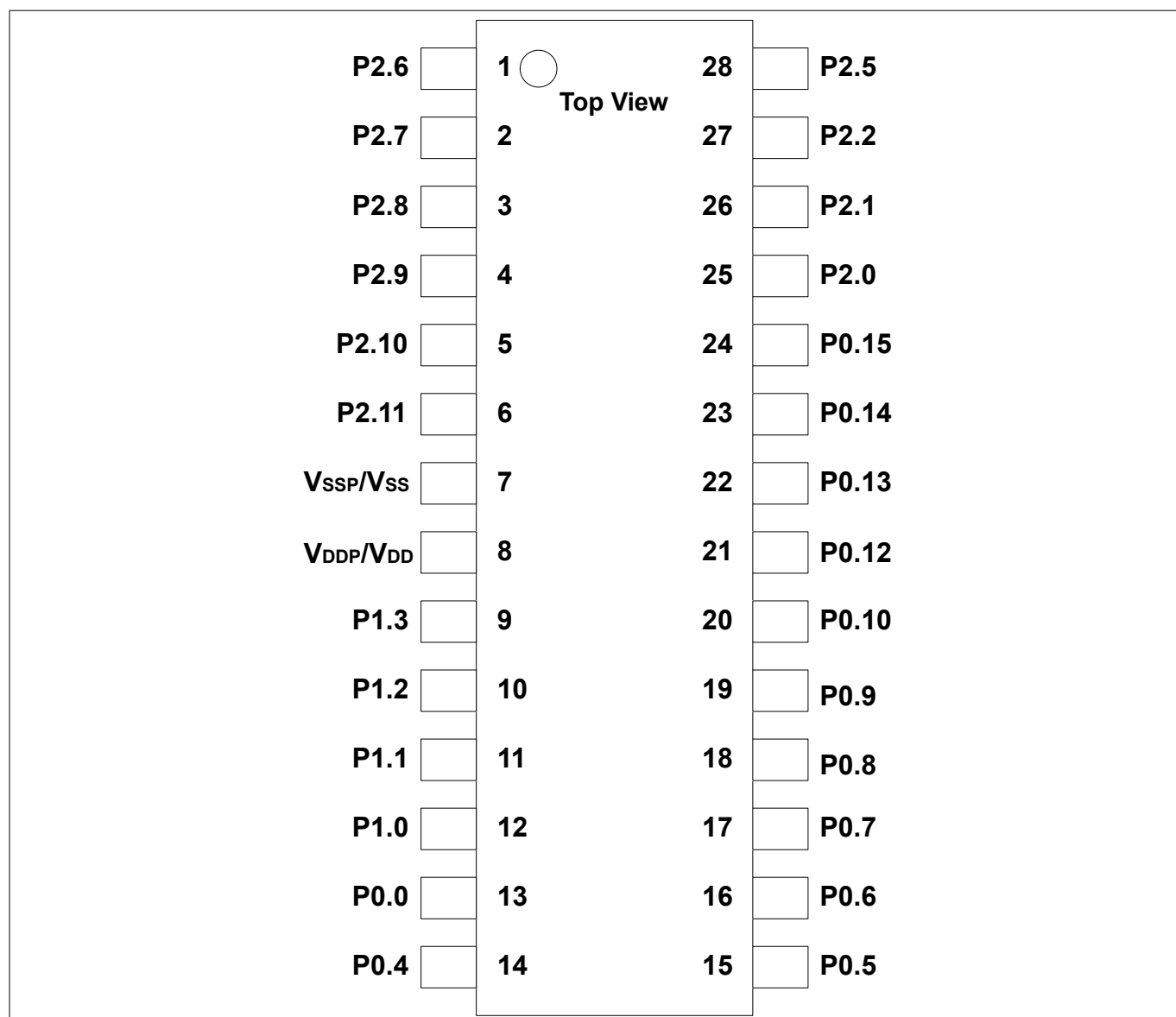
Figure 5 XMC1300 PG-TSSOP-28 Pin Configuration (top view)
