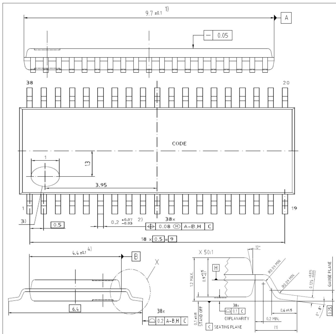
Figure 26 PG-TSSOP-38-9
