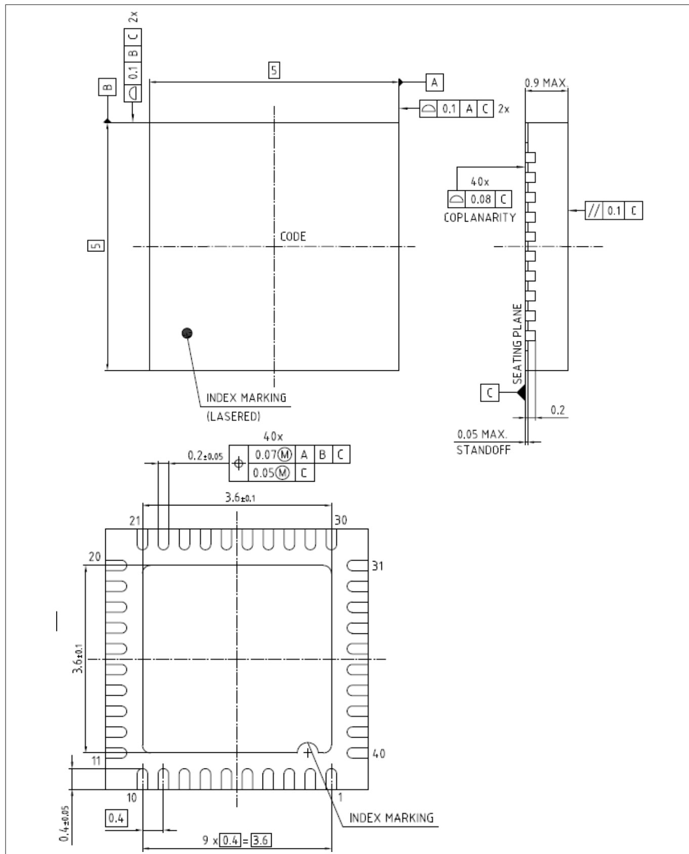
Figure 30 PG-VQFN-40-13
