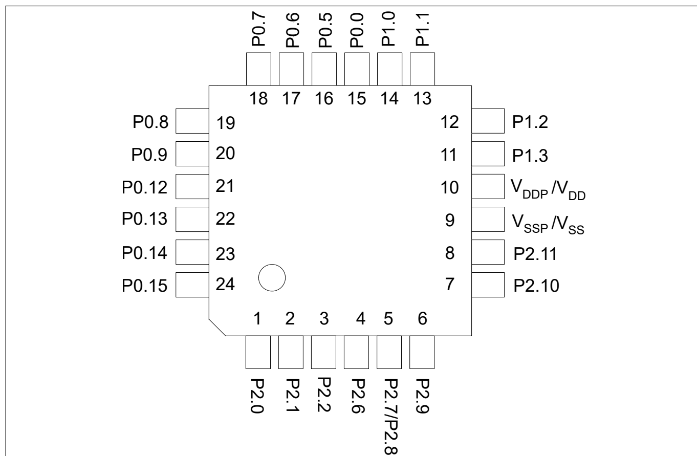
Figure 7 XMC1300 PG-VQFN-24 Pin Configuration (top view)
