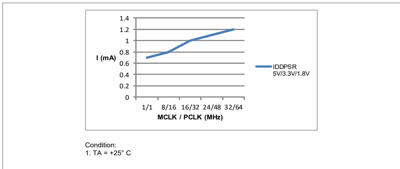
Figure 15 Sleep mode, peripherals clocks disabled, Flash powered down: Supply current I_{DDPSR} over supply voltage V_{DDP} for different clock frequencies
