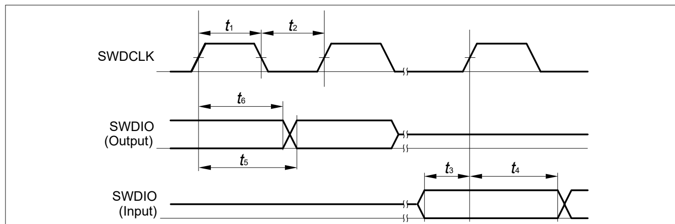
Figure 21 SWD Timing
