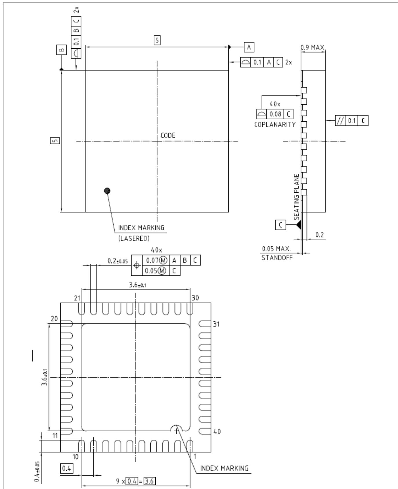
Figure 30 PG-VQFN-40-13
