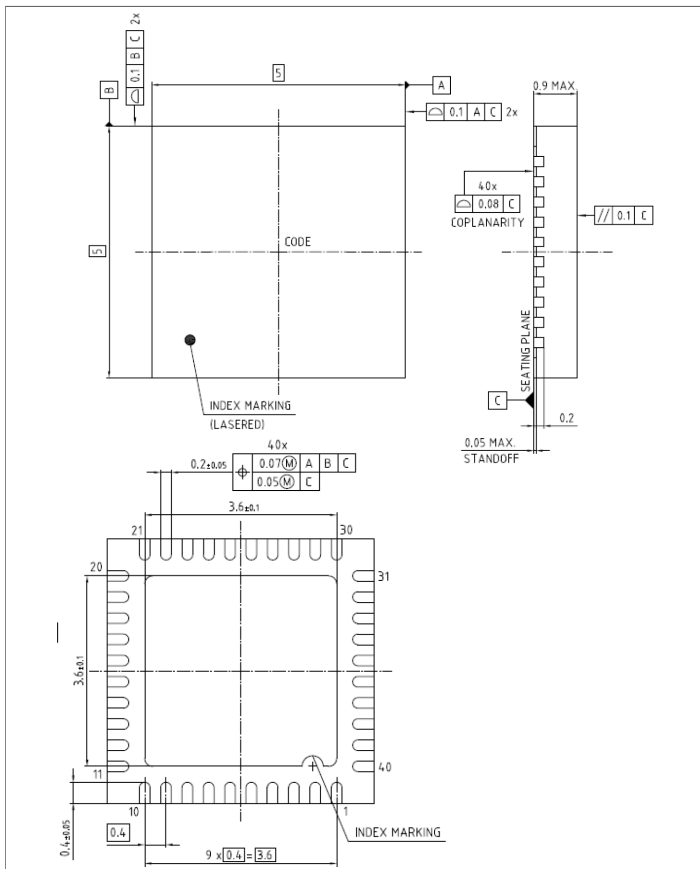
Figure 30 PG-VQFN-40-13
