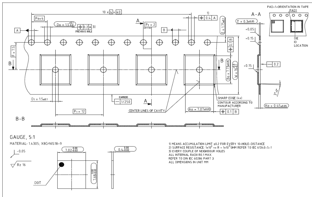
Figure 3-30 Carrier Tape Dimenions
