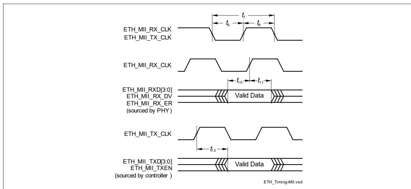
Figure 3-26 ETH MII Signal Timing
